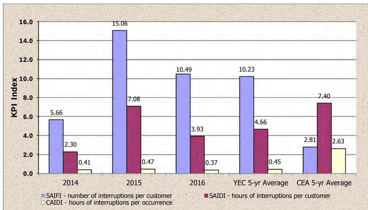
Figure 2-1: Yukon Energy Distribution KPIs: 2014 to 2016
