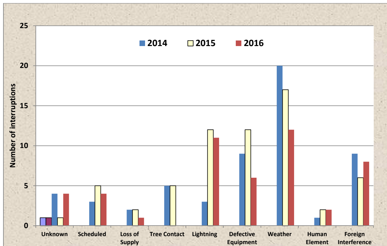
Figure 2-2: Causes of Interruptions: 2014 to 2016
