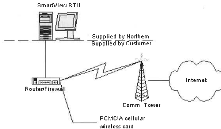
Figure 4-5 Cellular wireless Internet
