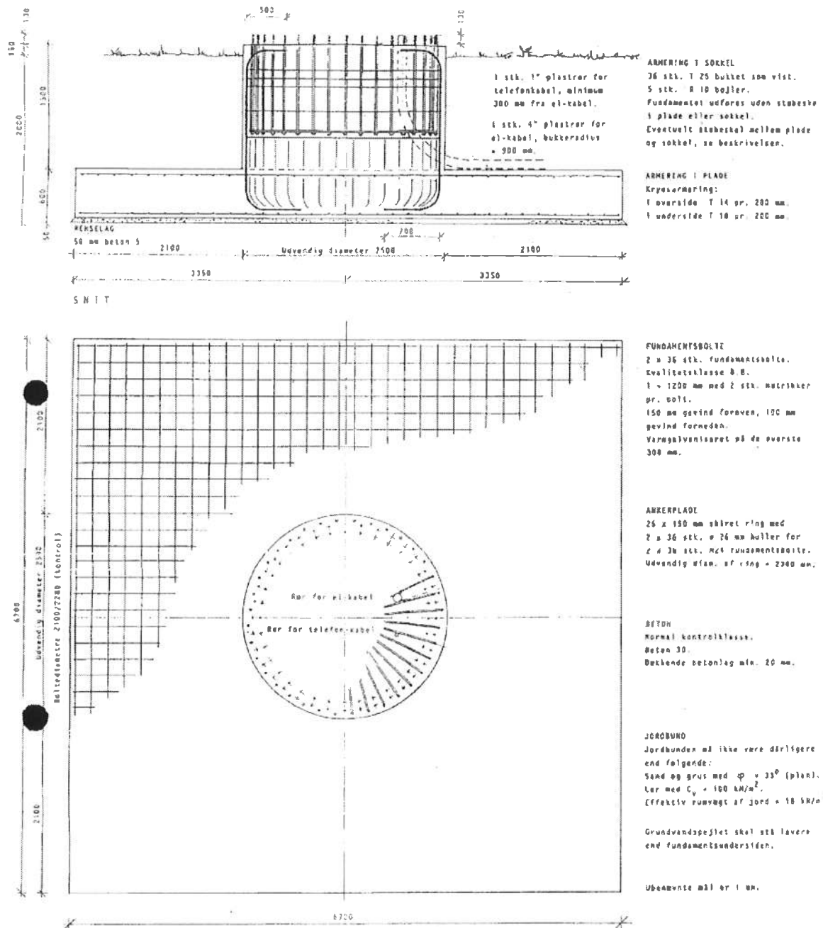
Figure 2. Example of foundation design
