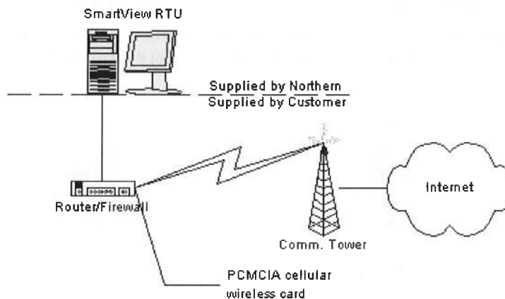
Figure 4-3 Customer LAN Internet
