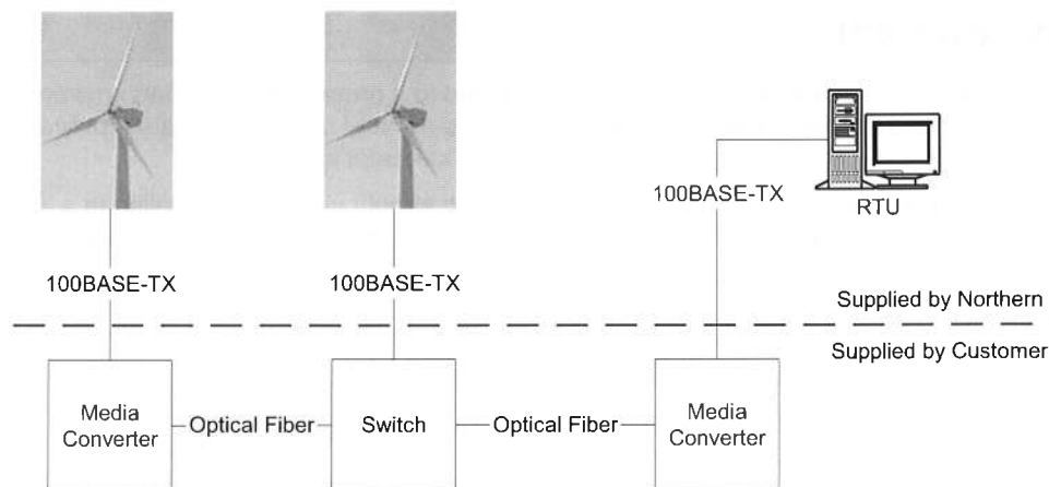
Figure 4-1 Fiber network
