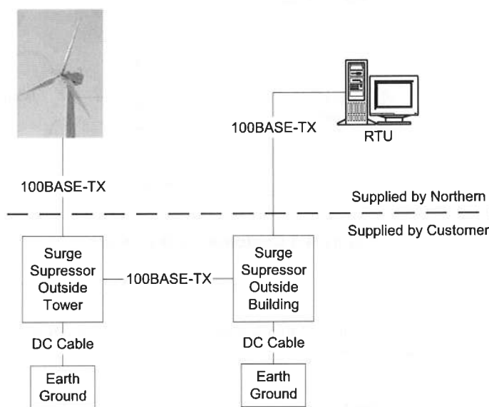
Figure 4-2 Copper network
