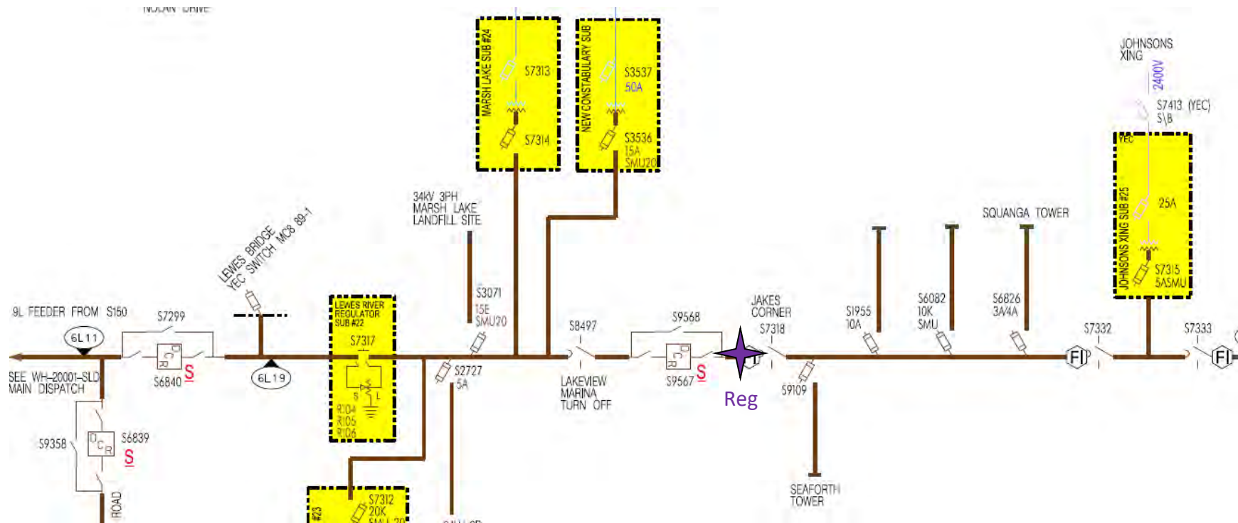
Figure 7: Alternative 3 Regulator Location SLD
