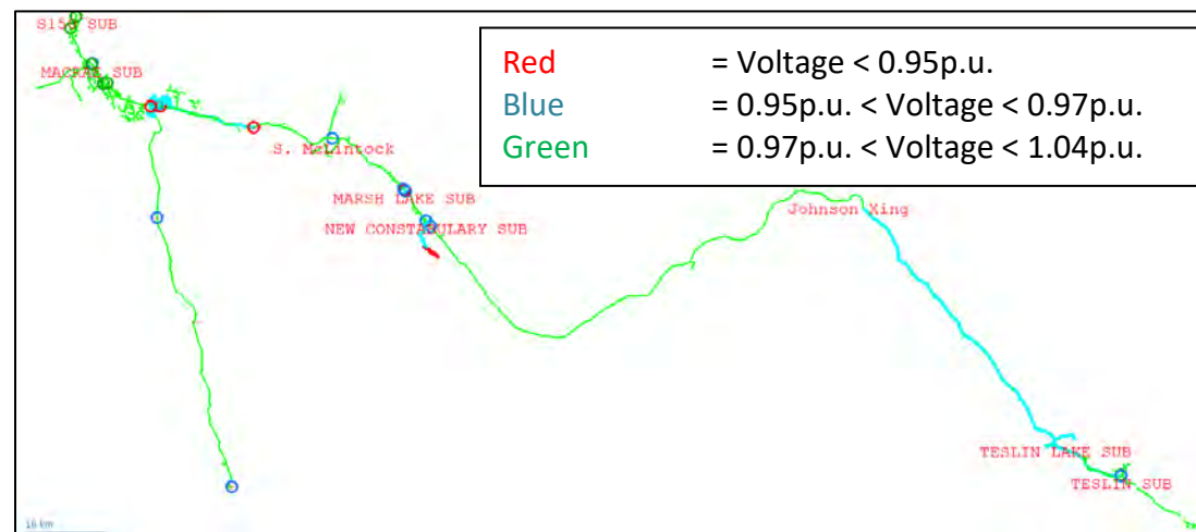
Figure 5: Alternative 2 Voltage Conditions
